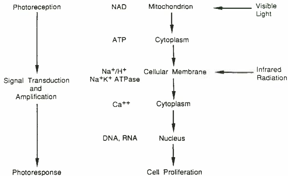
Figure 3. A model for the low level laser radiation stimulation of biological systems (modified from Karu 8 ). Biostimulation at 633 nm results from the absorption of light by components of the respiratory chain in the mitochondria (see text), which results in increased metabolism, which leads to signal transduction to other parts of the cell, and ultimately to the photoreponse. Because infrared radiation is expected to exert its photophysical effect on the molecules that make up cellular membranes (see text), an arrow has been added to suggest that infrared radiation produces the same final biological result as does 633 nm radiation, but the two radiations start the cascade of metabolic events at different levels
